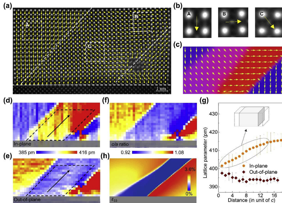
Fig. 2. Atomic structure of the a -domain. (a) An atomically resolved HAADF-STEM image of an a -domain in PbTiO 3 films overlaid with atomic displacement vectors. (b) Enlarged PbTiO 3 unit cells are averaged from the three marked areas in (a). (c) Phase-field modeling of polarization arrangements of the a -domain. (d) In-plane, (e) out-of-plane lattice parameters, and (f) c/a ratio maps of c/a/c domains. The SrRuO 3 electrode is indicated by a gray rectangular. (g) Profiles of the in-plane and out-of-plane lattice parameters in a -domain corresponding to the marked areas in (c) and (d). The inset indicates the reduced lattice c in a -domain. The error bar is the standard deviation (s.d.). (h) Simulate out-of-plane normal strain around the a -domain.
