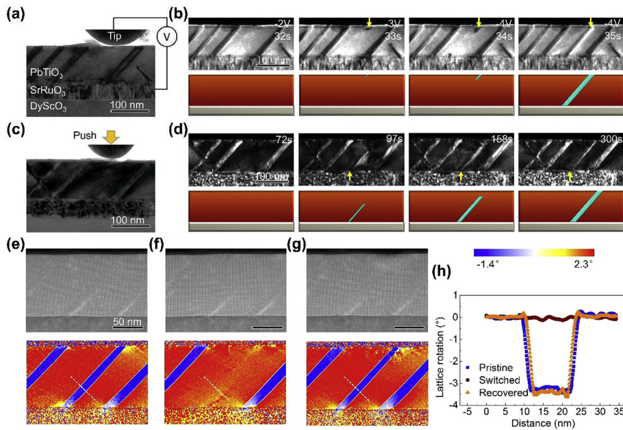
Fig. 4. Recovery of a -domains via electrical and mechanical stimuli. (a) A bright field TEM image of the domain structure. (b) A chronological image series showing the recovery process of a -domain by electric fields with schematics. (c) A bright field TEM image of the domain structure. The W tip acts as an indenter for mechanical loading. (d) A chronological image series showing the recovery of a -domain under mechanical excitation with schematics. HAADF-STEM images of the pristine (e), switched (f) and recovered (g) states of a -domain with lattice rotation maps obtained from GPA indicate the locally reversible switching of the individual a -domain. (h) Profiles of lattice rotation corresponding to the dashed lines in lattice rotation maps. The lattice rotation in c -domain far away from the domain wall is normalized to 0.
