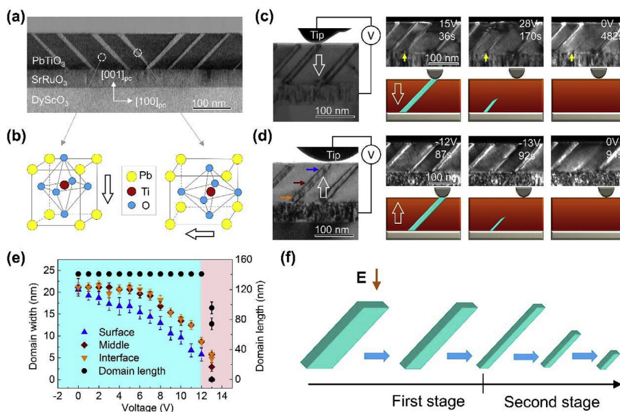
Fig. 1. Domain structure and electric field induced switching of an individual a -domain. (a) A STEM image of PbTiO 3 thin films grown on DyScO 3 with 50-nm-thick SrRuO 3 electrodes. (b) Schematics of the unit cells in c -domain with out-of-plane polarization and in a -domain with in-plane polarization. (c) A chronological TEM dark-field image series depicting the switching process of an a -domain under negative voltage. The SrRuO 3 electrode is grounded. (d) A chronological TEM dark-field image series depicting the switching process of an a -domain under positive voltage. The SrRuO 3 electrode is grounded. (e) The width and length of a -domain as a function of applied voltage. The width of a -domain in the bottom, middle and surface corresponding to the three marked arrows in (c). The dark circle shows the length of a -domain. (f) Schematic illustration of the two-stage switching process of an individual ferroelastic domain driven by electric fields.
